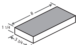
STANDARD PAVER
