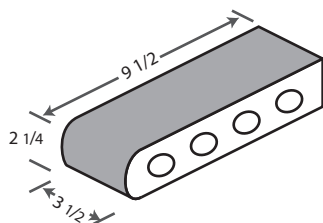
9" SINGLE BULLNOSE
