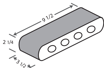
9" DOUBLE BULLNOSE
